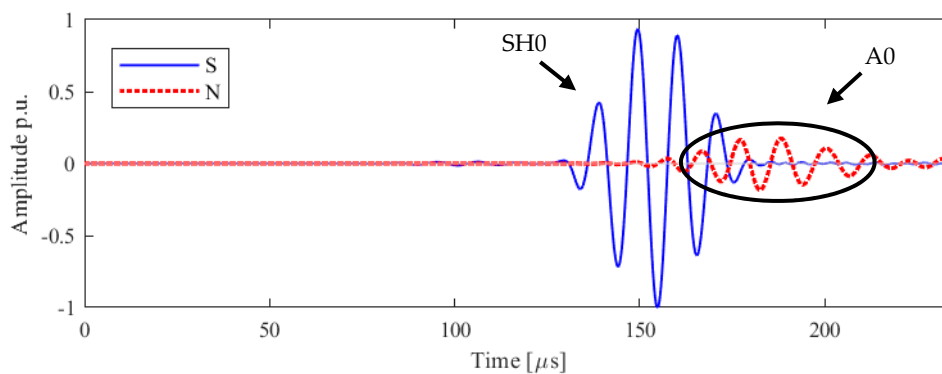
Figure 9. Configuration A numerical results of the in-plane (blue), 'S', and out-of-plane, 'N', (red) velocities along the line orthogonal to the line of vibration. Normalized data are shown: modes are identified and labelled accordingly.
