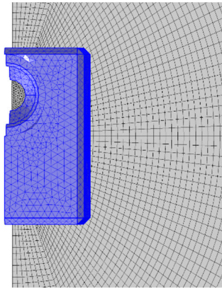
Figure 6. Picture showing the tetrahedral mesh on the transducer (highlighted in blue) and the quadratic mesh on the plate.
