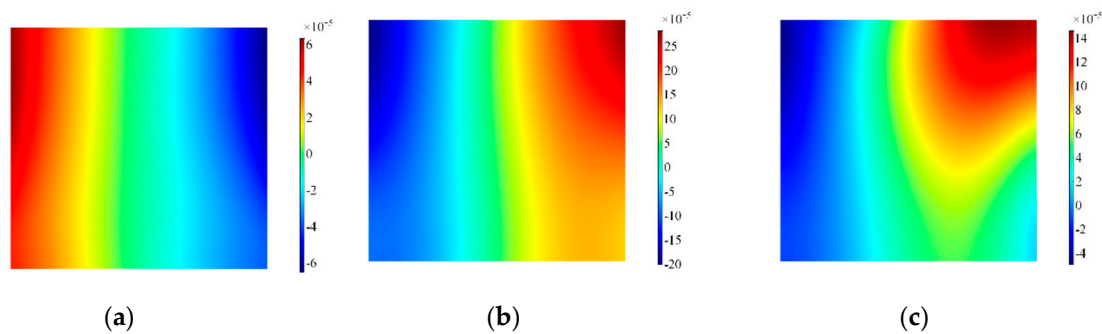
Figure 19. Surface plot for the out-of-plane velocity on the side of the backing mass, Configuration A'. Note that data are plotted at timeframes of 100 \mu s (a), 300 \mu s (b) and 500 \mu s (c).
