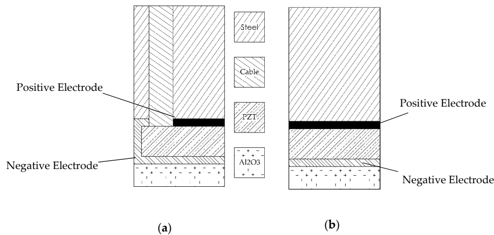
Figure 20. Transducer (a) Configuration A (wrap around electrodes) and (b) Configuration B (proposed modified electrode attachment and geometry). Note that configuration A presents an access hole for the electrical connectivity: positive electrode is presented with a thicker black line and negative electrode along the alumina layer. The representation is exaggerated to help the understanding.
