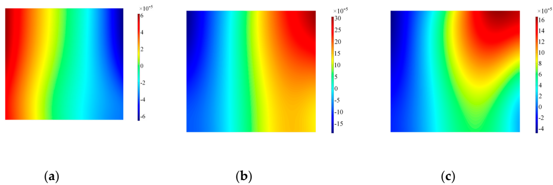
Figure 14. Surface plot for the out-of-plane velocity on the side of the backing mass, Configuration A. Note that data are plotted at timeframes of 100 \mu\text{s} (a), 300 \mu\text{s} (b) and 500 \mu\text{s} (c).
