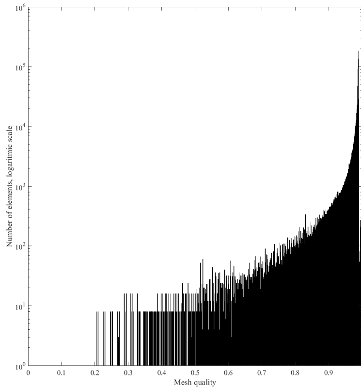
Figure 7. Plot of the number of elements as a function of mesh quality. Note that the ordinate axis is in logarithmic scale.
