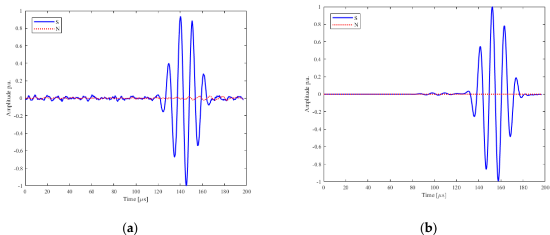
Figure 21. Configuration B results of the in-plane (blue), 'S', and out-of-plane, 'N', (red) velocities, experimental (a) and numerical (b) along the line orthogonal to the line of vibration. Amplitude and normalized data are shown.
