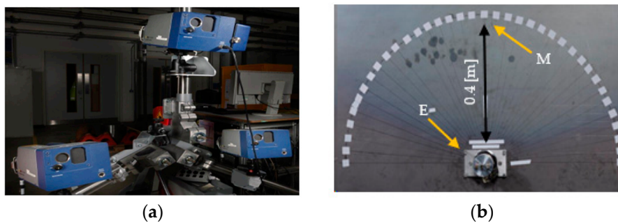
Figure 3. Laboratory experiments to characterize the transducers, 3D Laser Doppler Vibrometer used to monitor the surface vibration at the point of interest (a) PSV-400 3D Doppler Vibrometer used to monitor the surface vibration at the point of interest (b) experimental setup illustrating the point of excitation (labelled as E) and monitoring point (labelled as M) and the corresponding distance in meters.
