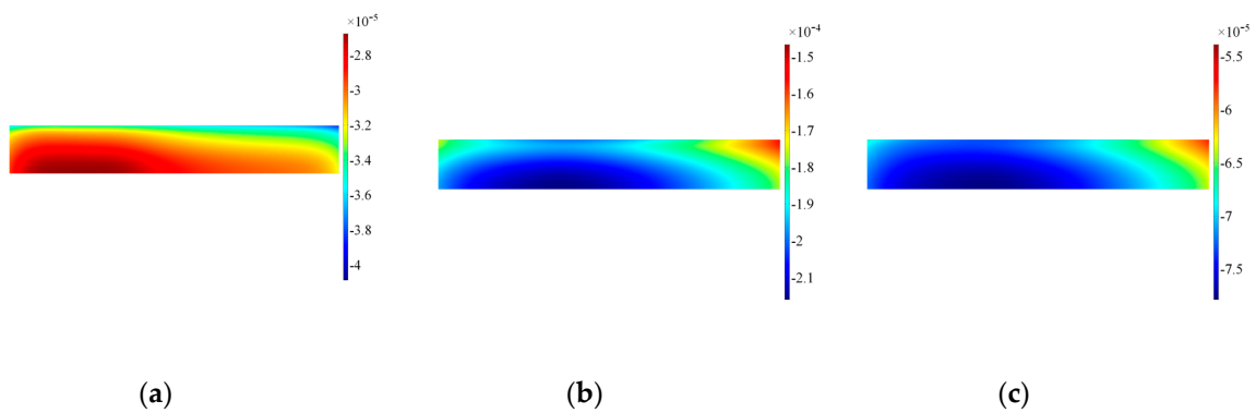
Figure 16. Surface plot for in-of-plane velocity on the alumina wear-plate, Configuration A'. Note that data are plotted at timeframes of 100 \mu s (a), 300 \mu s (b) and 500 \mu s (c).
