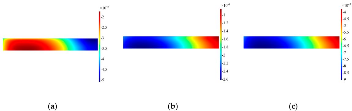
Figure 11. Surface plot for in-plane velocity on the alumina wear-plate, Configuration A. Note that data are plotted at timeframes of 100 \mu\text{s} (a), 300 \mu\text{s} (b) and 500 \mu\text{s} (c).
