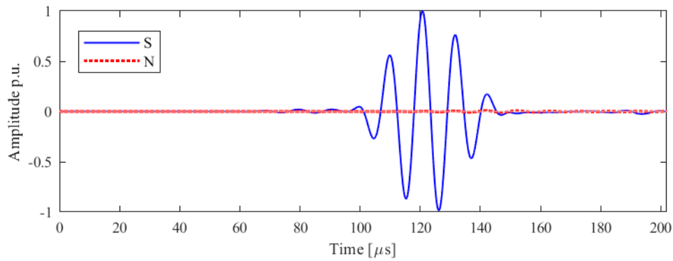
Figure 10. Point source numerical results of the in-plane (blue), ‘S’, and out-of-plane, ‘N’, (red) velocities along the line orthogonal to the line of vibration. Normalized data are shown.
