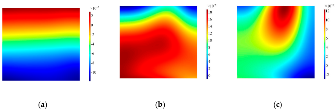
Figure 13. Surface plot for the in-plane velocity on the side of the backing mass, Configuration A. Note that data are plotted at timeframes of 100 \mu s (a), 300 \mu s (b) and 500 \mu s (c).
