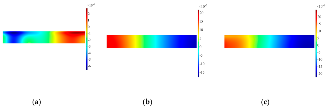
Figure 17. Surface plot for out-of-plane velocity on the alumina wear-plate, Configuration A'. Note that data are plotted at timeframes of 100 \mu s (a), 300 \mu s (b) and 500 \mu s (c).
