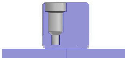
Figure 5. Picture showing the symmetry condition imposed on the transducer and on the plate, highlighted in blue.
