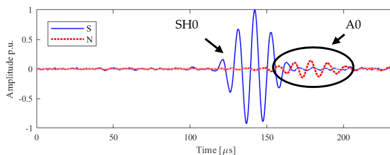
Figure 4. Laboratory experiments of the in-plane (blue), ‘S’, and out-of-plane, ‘N’, (red) velocities along the line orthogonal to the axis of vibration, for Configuration A. Normalized data are shown: modes are identified and labelled accordingly.
