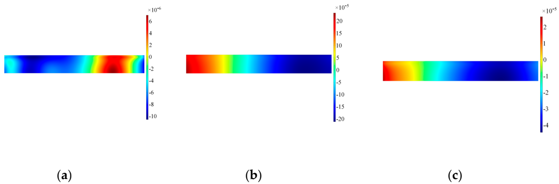
Figure 12. Surface plot for out-of-plane velocity on the alumina wear-plate, Configuration A. Note that data are plotted at timeframes of 100 \mu s (a), 300 \mu s (b) and 500 \mu s (c).
