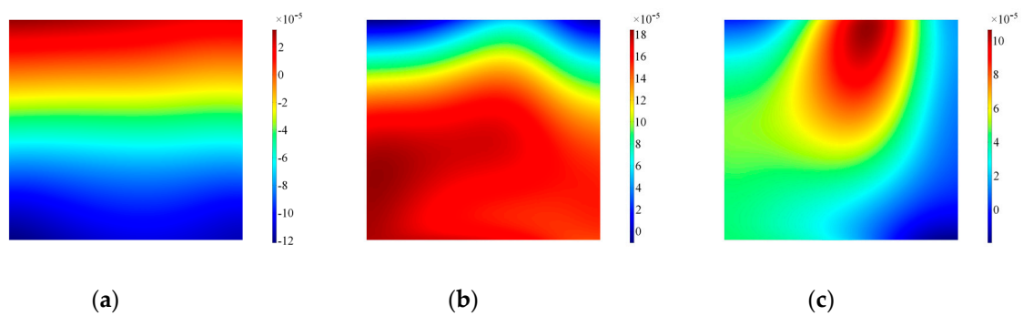
Figure 18. Surface plot for the in-plane velocity on the side of the backing mass, Configuration A'. Note that data are plotted at timeframes of 100 \mu s (a), 300 \mu s (b) and 500 \mu s (c).
