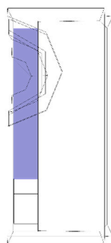
Figure 2. Imported CAD of the transducer viewed from top. Due to symmetry along the longitudinal axis only half the transducer is shown. Backing mass is in mechanical and electrical contact with the piezoelectric element. The actuation area on the top electrode of the piezoelectric element is highlighted in blue (it doesn't extend to the full length of the transducer due to the wrapped around electrode, configuration A). The access cable is cleared from internal electrical connection.
