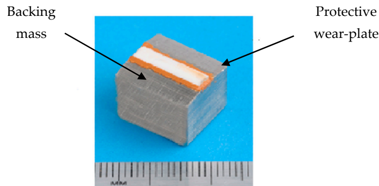
Figure 1. Current state-of-the-art transducer typical of those found with wrapped around electrodes. Labels are inserted to indicate the two features visible externally, the backing mass and the protective wear-plate.
