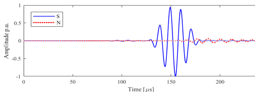
Figure 15. Configuration A' results of the in-plane (blue), 'S', and out-of-plane, 'N', (red) velocities along the line orthogonal to the line of vibration. Normalized data are shown.
